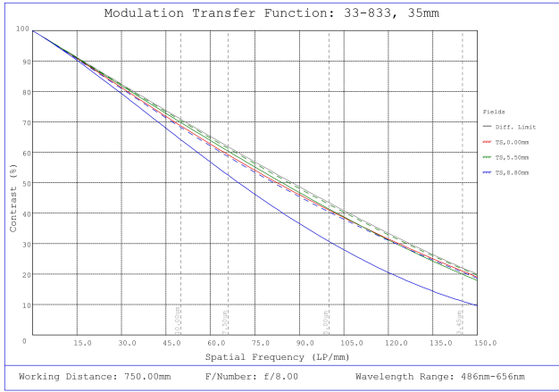
#33-833, 35mm f/8.0, HPI Series Fixed Focal Length Lens, Modulated Transfer Function (MTF) Plot, 750mm Working Distance, f8
