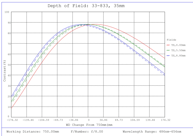
#33-833, 35mm f/8.0, HPI Series Fixed Focal Length Lens, Depth of Field Plot, 750mm Working Distance, f8
