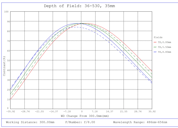
#36-530, 35mm f/8.0, HPr Series Fixed Focal Length Lens, Depth of Field Plot, 300mm Working Distance, f8
