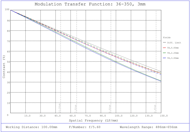
#36-350, 3mm FL f/5.6, Rugged Blue Series M12 Lens, Modulated Transfer Function (MTF) Plot, 100mm Working Distance, f5.6
