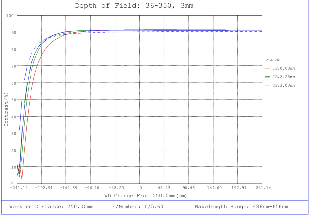
#36-350, 3mm FL f/5.6, Rugged Blue Series M12 Lens, Depth of Field Plot, 250mm Working Distance, f5.6
