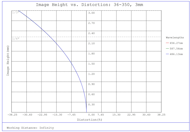
#36-350, 3mm FL f/5.6, Rugged Blue Series M12 Lens, Distortion Plot
