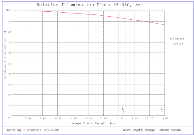
#36-350, 3mm FL f/5.6, Rugged Blue Series M12 Lens, Relative Illumination Plot
