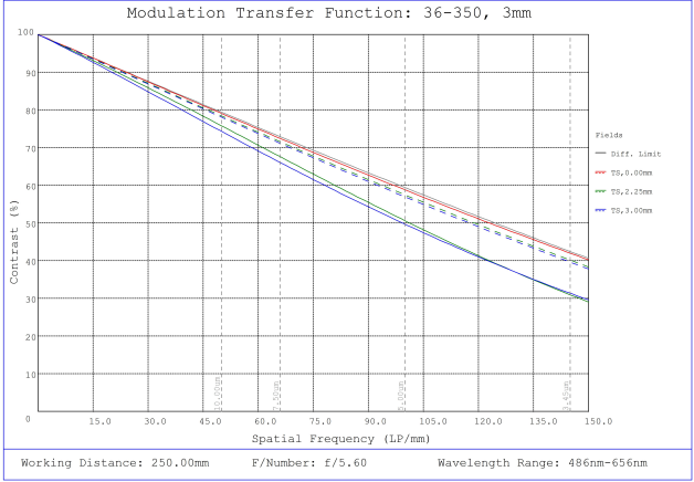
#36-350, 3mm FL f/5.6, Rugged Blue Series M12 Lens, Modulated Transfer Function (MTF) Plot, 250mm Working Distance, f5.6
