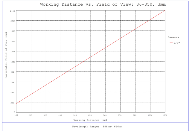
#36-350, 3mm FL f/5.6, Rugged Blue Series M12 Lens, Working Distance versus Field of View Plot
