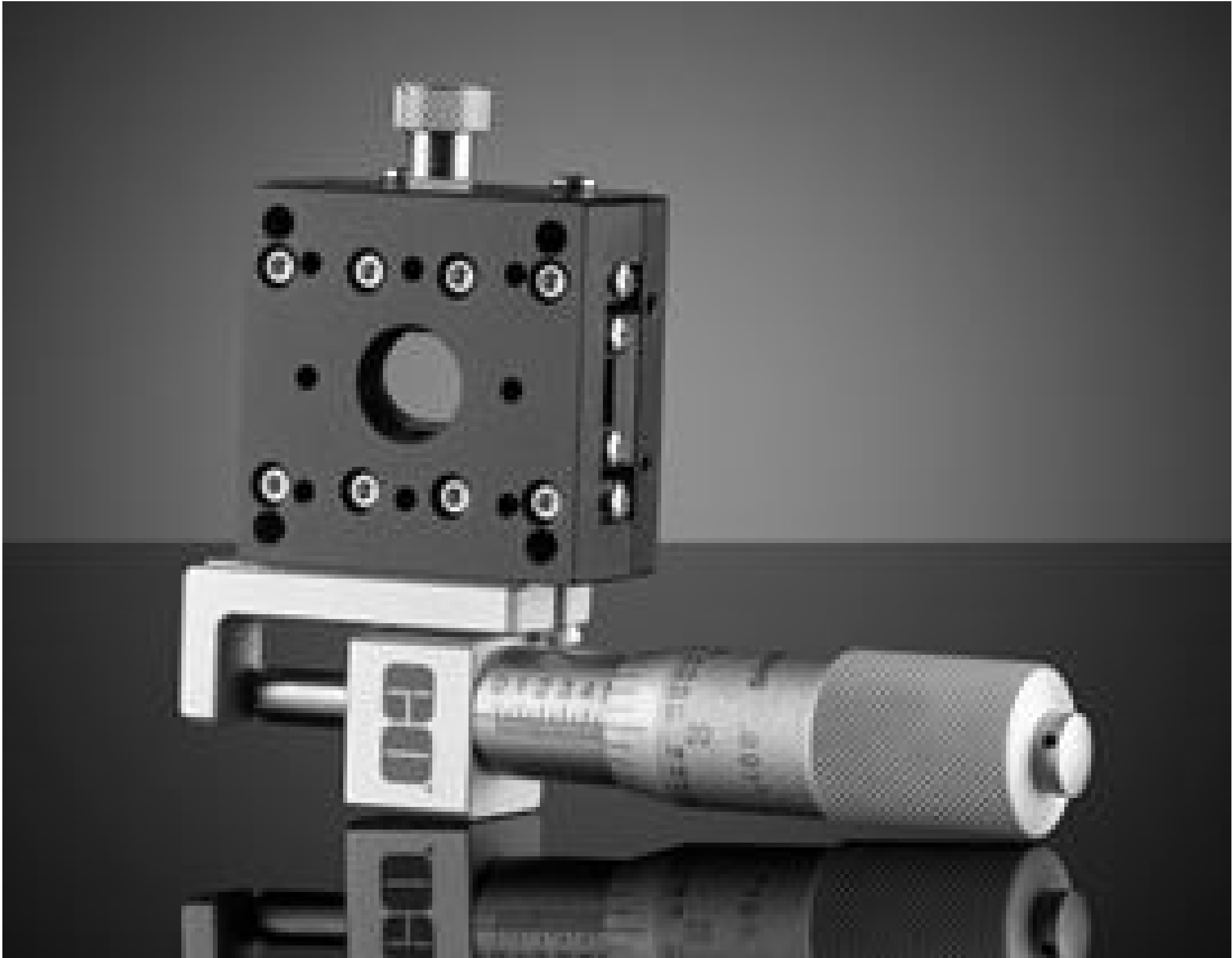
40mm, Side Drive, Thru-Hole Micrometer Stage
