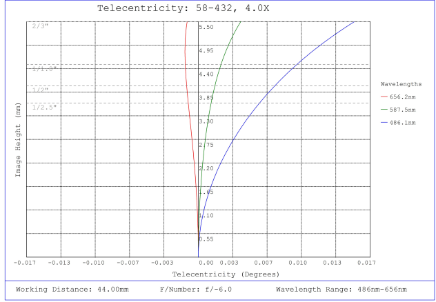
#58-432, 4.0X SilverTL™ Telecentric Lens, Telecentricity Plot
