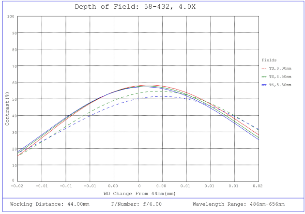
#58-432, 4.0X SilverTL™ Telecentric Lens, Depth of Field Plot, 44mm Working Distance, f6
