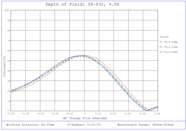
#58-432, 4.0X SilverTL™ Telecentric Lens, Depth of Field Plot, 44mm Working Distance, f10
