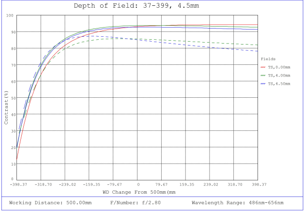
#37-399, 4.5mm, f/2.8 Cr Series Fixed Focal Length Lens, Depth of Field Plot, 500mm Working Distance, f2.8
