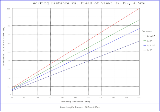
#37-399, 4.5mm, f/2.8 Cr Series Fixed Focal Length Lens, Working Distance versus Field of View Plot
