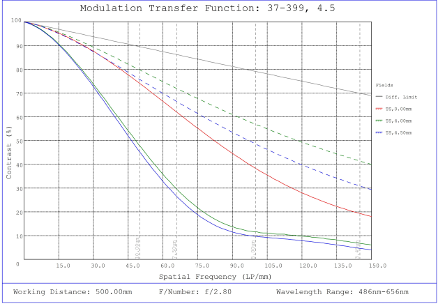
#37-399, 4.5mm, f/2.8 Cr Series Fixed Focal Length Lens, Modulated Transfer Function (MTF) Plot, 500mm Working Distance, f2.8
