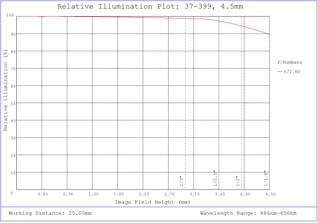
#37-399, 4.5mm, f/2.8 Cr Series Fixed Focal Length Lens, Relative Illumination Plot
