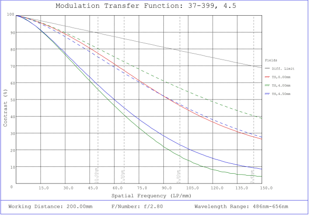
#37-399, 4.5mm, f/2.8 Cr Series Fixed Focal Length Lens, Modulated Transfer Function (MTF) Plot, 200mm Working Distance, f2.8
