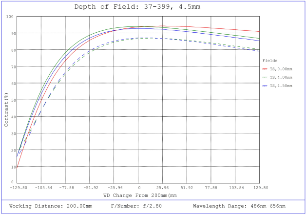
#37-399, 4.5mm, f/2.8 Cr Series Fixed Focal Length Lens, Depth of Field Plot, 200mm Working Distance, f2.8
