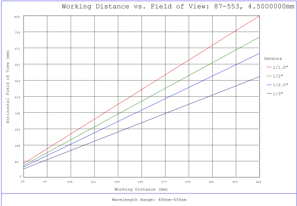
#87-553, 4.5mm, f/4 Ci Series Fixed Focal Length Lens, Working Distance versus Field of View Plot
