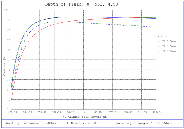
#87-553, 4.5mm, f/4 Ci Series Fixed Focal Length Lens, Depth of Field Plot, 500mm Working Distance, f4
