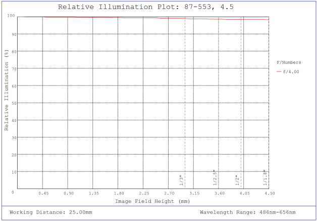
#87-553, 4.5mm, f/4 Ci Series Fixed Focal Length Lens, Relative Illumination Plot
