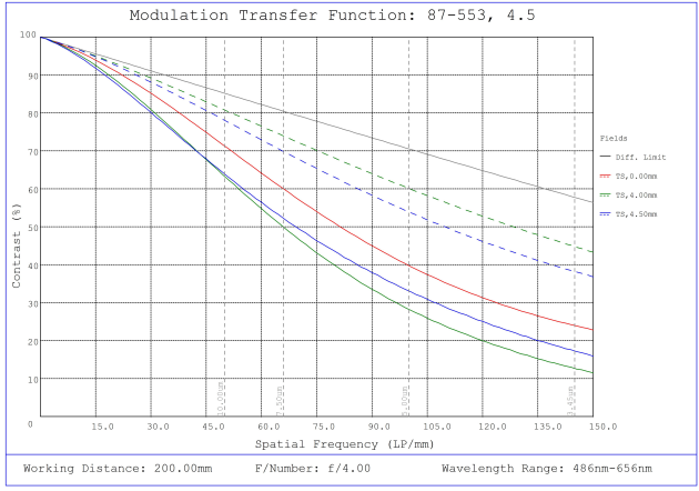
#87-553, 4.5mm, f/4 Ci Series Fixed Focal Length Lens, Modulated Transfer Function (MTF) Plot, 200mm Working Distance, f4
