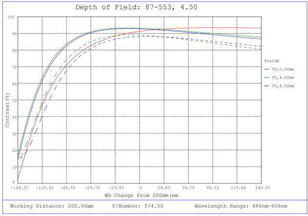
#87-553, 4.5mm, f/4 Ci Series Fixed Focal Length Lens, Depth of Field Plot, 200mm Working Distance, f4
