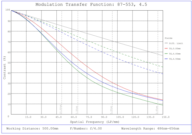
#87-553, 4.5mm, f/4 Ci Series Fixed Focal Length Lens, Modulated Transfer Function (MTF) Plot, 500mm Working Distance, f4
