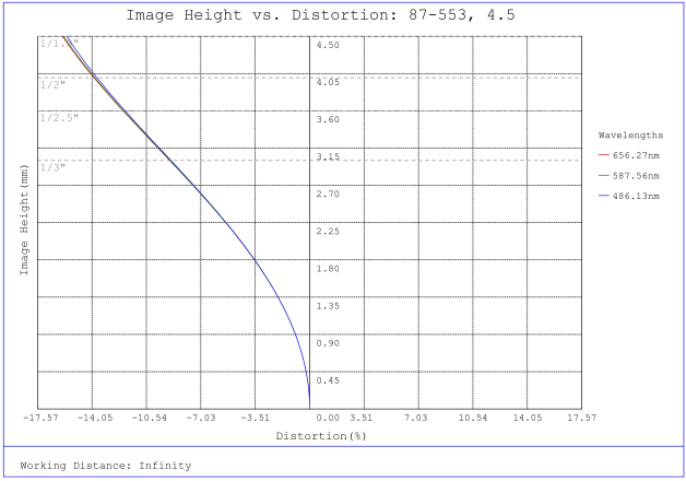
#87-553, 4.5mm, f/4 Ci Series Fixed Focal Length Lens, Distortion Plot
