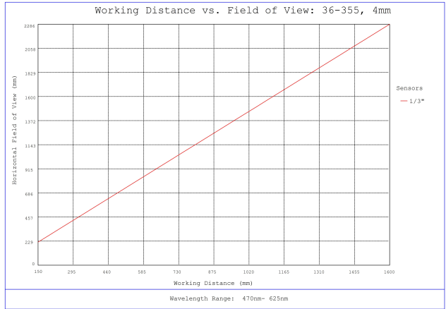
#36-355, 4mm FL f/8, Rugged Blue Series M12 Lens, Working Distance versus Field of View Plot
