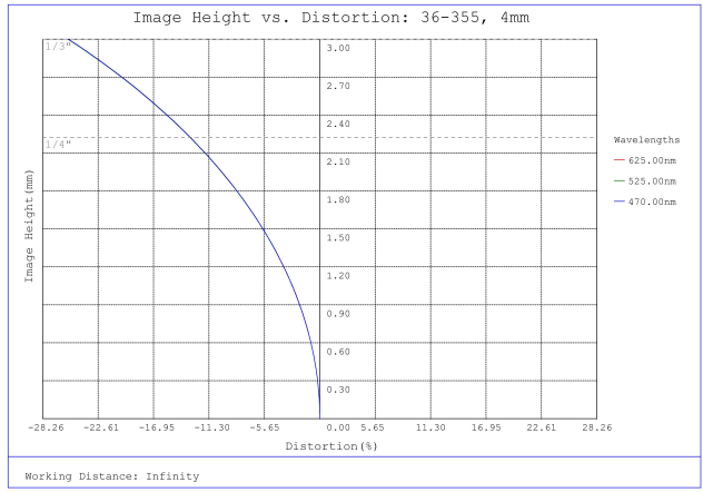
#36-355, 4mm FL f/8, Rugged Blue Series M12 Lens, Distortion Plot
