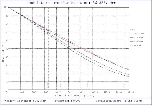
#36-355, 4mm FL f/8, Rugged Blue Series M12 Lens, Modulated Transfer Function (MTF) Plot, 500mm Working Distance, f8
