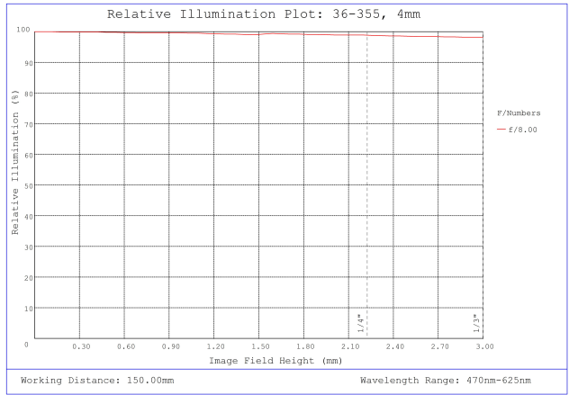
#36-355, 4mm FL f/8, Rugged Blue Series M12 Lens, Relative Illumination Plot
