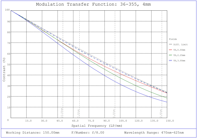
#36-355, 4mm FL f/8, Rugged Blue Series M12 Lens, Modulated Transfer Function (MTF) Plot, 150mm Working Distance, f8
