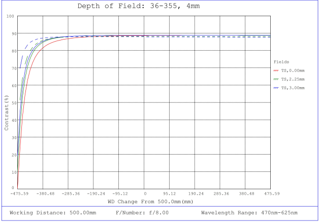
#36-355, 4mm FL f/8, Rugged Blue Series M12 Lens, Depth of Field Plot, 500mm Working Distance, f8
