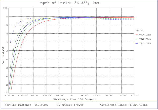
#36-355, 4mm FL f/8, Rugged Blue Series M12 Lens, Depth of Field Plot, 150mm Working Distance, f8
