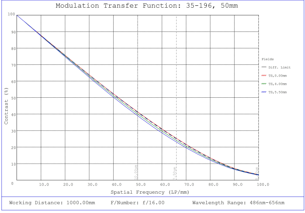
#35-196, 50mm, f/16 Cr Series Fixed Focal Length Lens, Modulated Transfer Function (MTF) Plot, 1000mm Working Distance, f16
