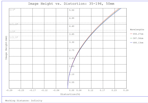
#35-196, 50mm, f/16 Cr Series Fixed Focal Length Lens, Distortion Plot
