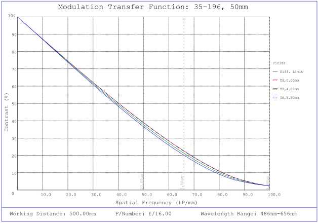
#35-196, 50mm, f/16 Cr Series Fixed Focal Length Lens, Modulated Transfer Function (MTF) Plot, 500mm Working Distance, f16
