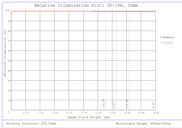
#35-196, 50mm, f/16 Cr Series Fixed Focal Length Lens, Relative Illumination Plot
