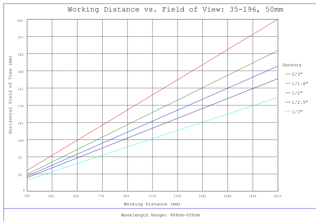
#35-196, 50mm, f/16 Cr Series Fixed Focal Length Lens, Working Distance versus Field of View Plot
