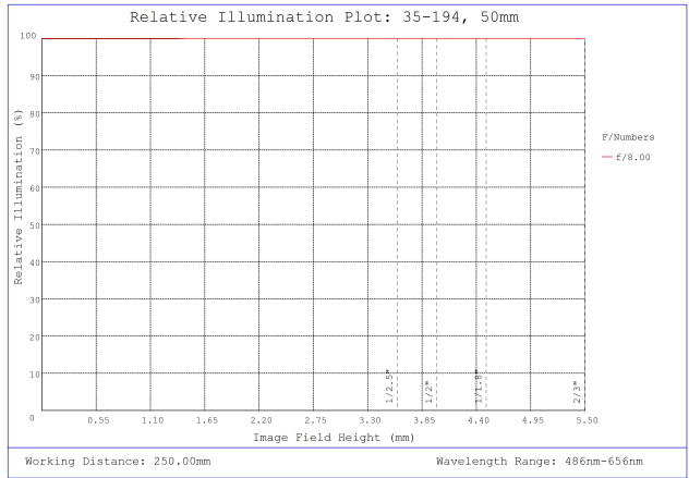
#35-194, 50mm, f/8.0 Cr Series Fixed Focal Length Lens, Relative Illumination Plot
