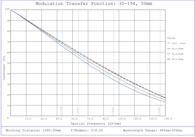
#35-194, 50mm, f/8.0 Cr Series Fixed Focal Length Lens, Modulated Transfer Function (MTF) Plot, 1000mm Working Distance, f8
