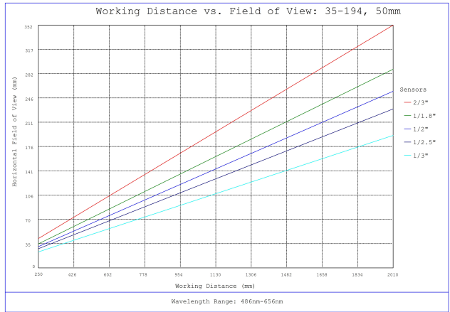
#35-194, 50mm, f/8.0 Cr Series Fixed Focal Length Lens, Working Distance versus Field of View Plot
