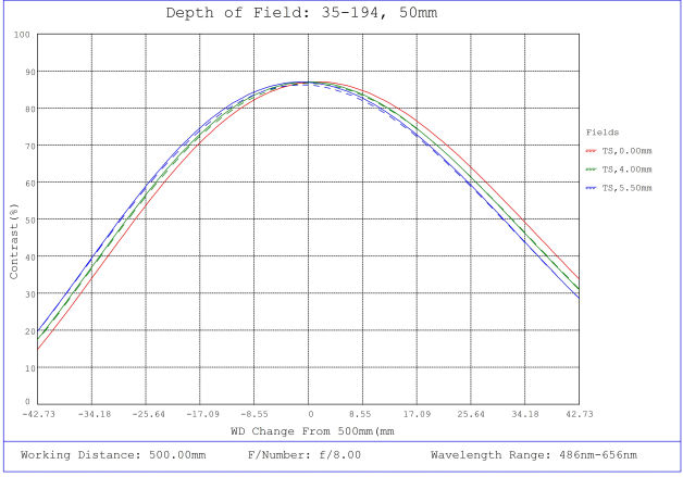
#35-194, 50mm, f/8.0 Cr Series Fixed Focal Length Lens, Depth of Field Plot, 500mm Working Distance, f8
