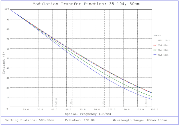
#35-194, 50mm, f/8.0 Cr Series Fixed Focal Length Lens, Modulated Transfer Function (MTF) Plot, 500mm Working Distance, f8
