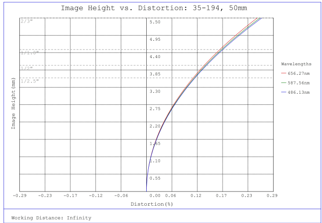
#35-194, 50mm, f/8.0 Cr Series Fixed Focal Length Lens, Distortion Plot
