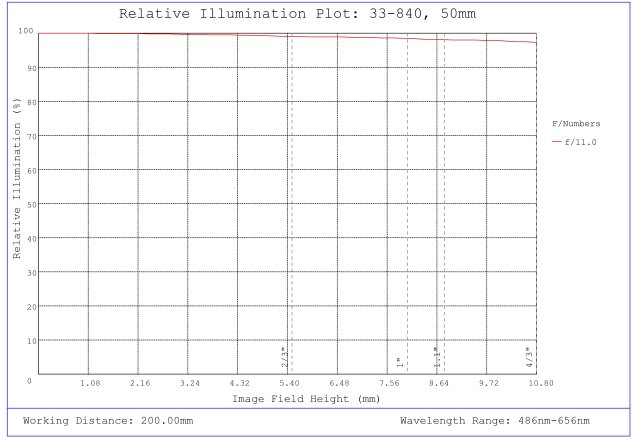
#33-840, 50mm f/11, HPI Series Fixed Focal Length Lens, Relative Illumination Plot
