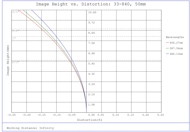
#33-840, 50mm f/11, HPI Series Fixed Focal Length Lens, Distortion Plot
