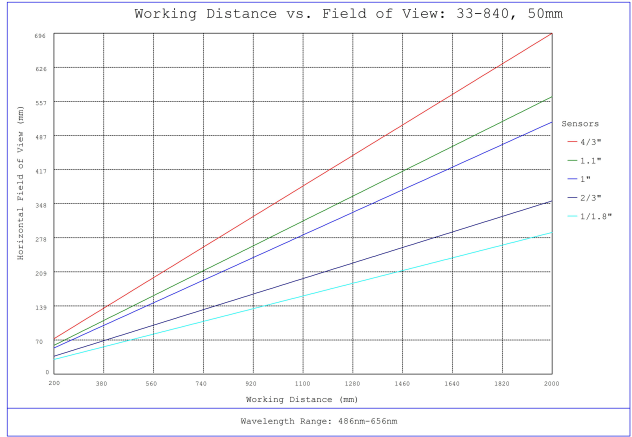
#33-840, 50mm f/11, HPI Series Fixed Focal Length Lens, Working Distance versus Field of View Plot
