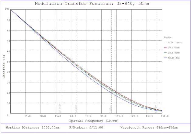
#33-840, 50mm f/11, HPi Series Fixed Focal Length Lens, Modulated Transfer Function (MTF) Plot, 1000mm Working Distance, f11
