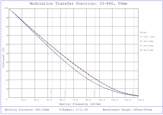
#33-840, 50mm f/11, HPi Series Fixed Focal Length Lens, Modulated Transfer Function (MTF) Plot, 400mm Working Distance, f11
