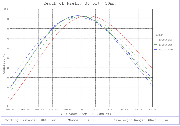
#36-534, 50mm f/4.0, HPr Series Fixed Focal Length Lens, Depth of Field Plot, 1000mm Working Distance, f4
