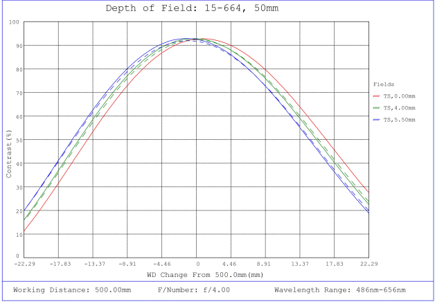
#15-664, 50mm, f/4.0 Sealed Cw Series Fixed Focal Length Lens, Depth of Field Plot, 500mm Working Distance, f4
