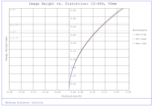
#15-664, 50mm, f/4.0 Sealed Cw Series Fixed Focal Length Lens, Distortion Plot
