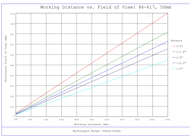
#86-617, 50mm, f/5.6 Ci Series Fixed Focal Length Lens, Working Distance versus Field of View Plot
