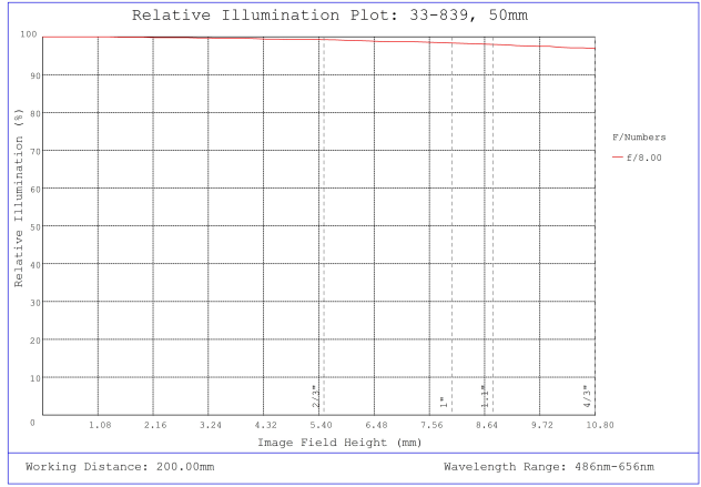
#33-839, 50mm f/8.0, HPi Series Fixed Focal Length Lens, Relative Illumination Plot
