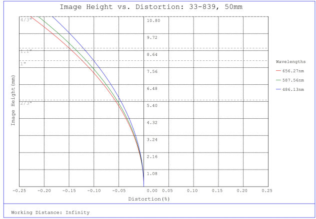
#33-839, 50mm f/8.0, HPi Series Fixed Focal Length Lens, Distortion Plot
