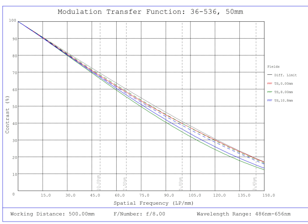
#36-536, 50mm f/8.0, HPr Series Fixed Focal Length Lens, Modulated Transfer Function (MTF) Plot, 500mm Working Distance, f8
