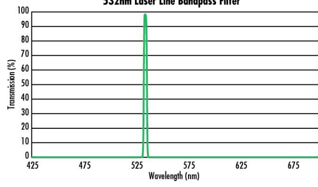
532nm Laser Line Bandpass Filter
