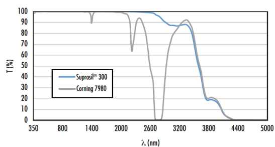
Internal Transmission (5mm Thick Samples)
