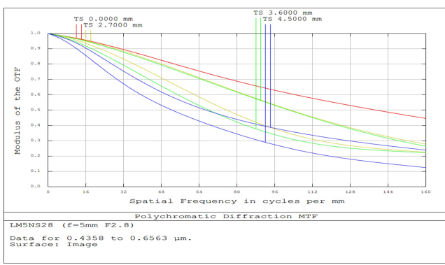
5mm FL, f/2.8, Low Distortion M12 Lens, MTF Plot
