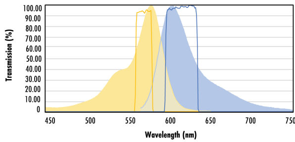
Legend: ROX Excitation Filter Typical, ROX Emission Filter Type, ROX Absorption, ROX Emission Overlay ROX Absorption and Emission with Excitation and Emission
