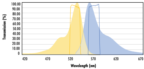
Legend: HEX Excitation Filter Typical, HEX Emission Filter Type, HEX Absorption, HEX Emission Overlay HEX Absorption and Emission with Excitation and Emission Filters
