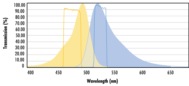
Legend: FAM Excitation Filter Typical, FAM Emission Filter Type, FAM Absorption, FAM Emission Overlay FAM Absorption & Emission with Excitation and Emission Filters
