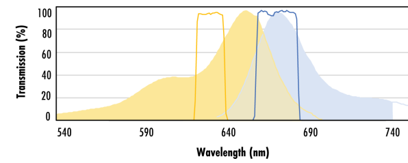
Legend: Cy5 Excitation Filter Typical, Cy5 Emission Filter Typical, Cy5 Absorption, Cy5 Emission Overlay Cy5 Absorption and Emission with Excitation and Emission Filters
