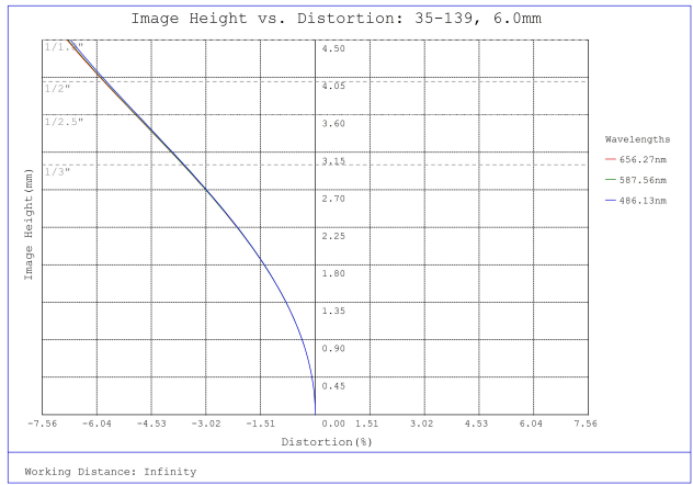
#35-139, 6mm, f/1.4 Cr Series Fixed Focal Length Lens, Distortion Plot
