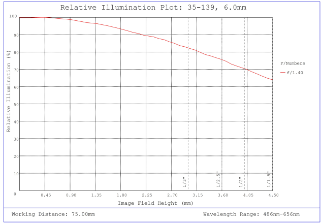
#35-139, 6mm, f/1.4 Cr Series Fixed Focal Length Lens, Relative Illumination Plot
