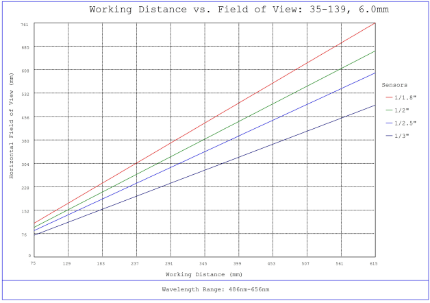
#35-139, 6mm, f/1.4 Cr Series Fixed Focal Length Lens, Working Distance versus Field of View Plot
