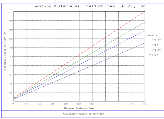
#86-596, 6mm, f/8 Ci Series Fixed Focal Length Lens, Working Distance versus Field of View Plot
