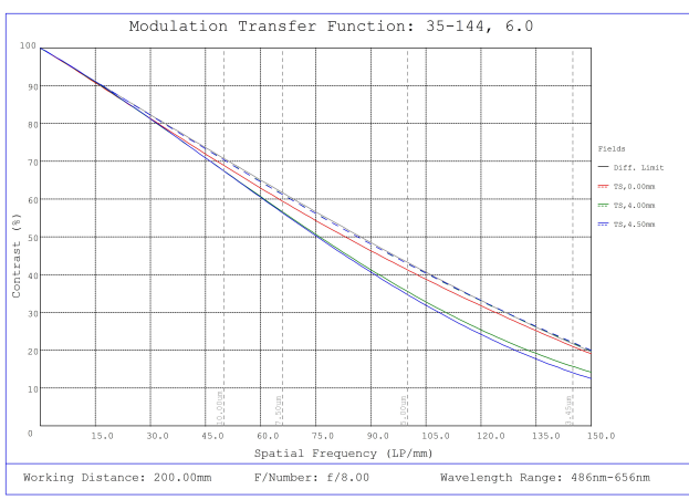
#35-144, 6mm, f/8 Cr Series Fixed Focal Length Lens, Modulated Transfer Function (MTF) Plot, 200mm Working Distance, f8
