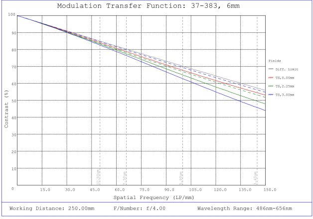
#37-383, 6mm FL f/4.0, Rugged Blue Series M12 Lens, Modulated Transfer Function (MTF) Plot, 250mm Working Distance, f4
