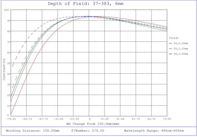
#37-383, 6mm FL f/4.0, Rugged Blue Series M12 Lens, Depth of Field Plot, 150mm Working Distance, f4
