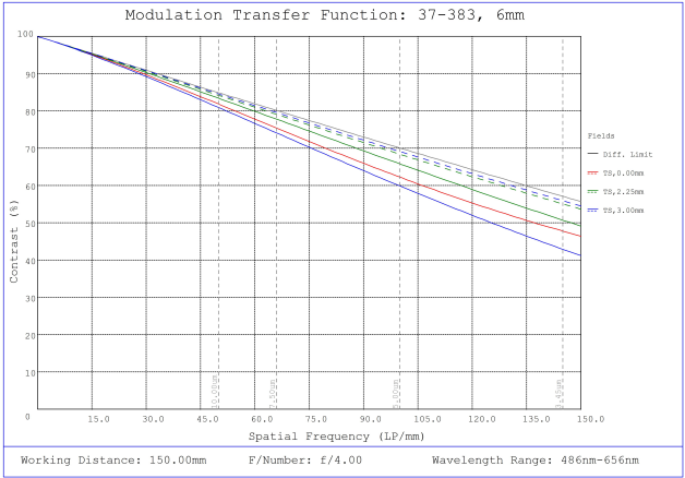
#37-383, 6mm FL f/4.0, Rugged Blue Series M12 Lens, Modulated Transfer Function (MTF) Plot, 150mm Working Distance, f4
