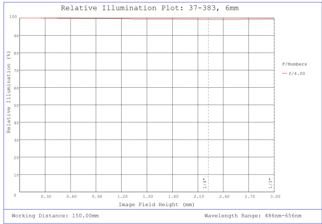
#37-383, 6mm FL f/4.0, Rugged Blue Series M12 Lens, Relative Illumination Plot
