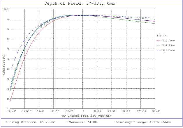
#37-383, 6mm FL f/4.0, Rugged Blue Series M12 Lens, Depth of Field Plot, 250mm Working Distance, f4
