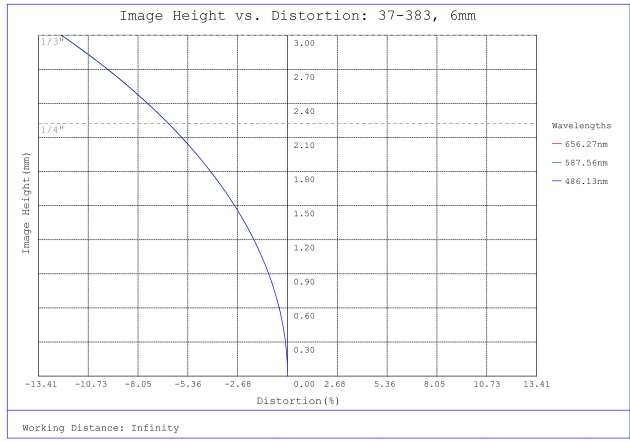
#37-383, 6mm FL f/4.0, Rugged Blue Series M12 Lens, Distortion Plot
