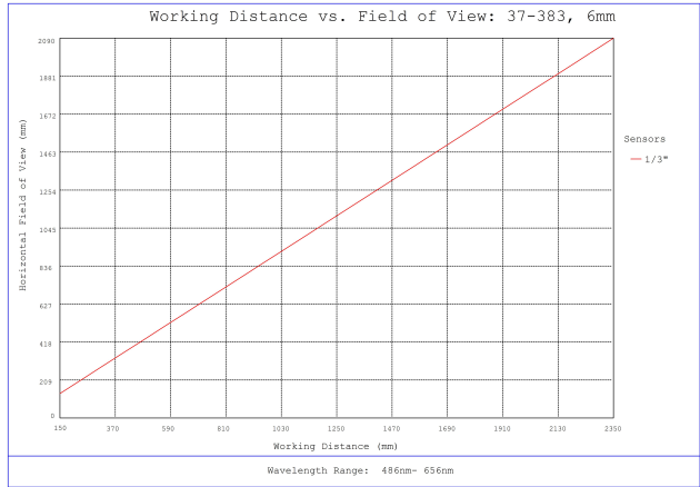
#37-383, 6mm FL f/4.0, Rugged Blue Series M12 Lens, Working Distance versus Field of View Plot
