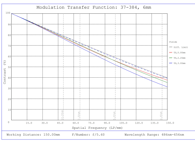
#37-384, 6mm FL f/5.6, Rugged Blue Series M12 Lens, Modulated Transfer Function (MTF) Plot, 150mm Working Distance, f5.6
