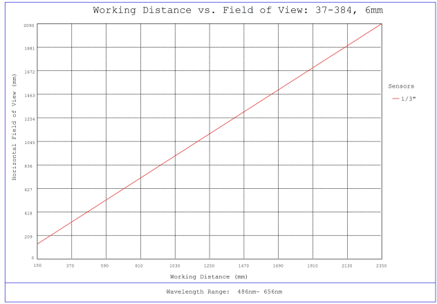
#37-384, 6mm FL f/5.6, Rugged Blue Series M12 Lens, Working Distance versus Field of View Plot
