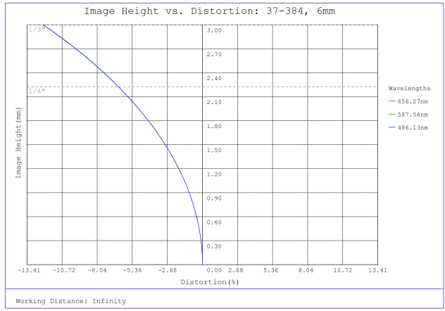
#37-384, 6mm FL f/5.6, Rugged Blue Series M12 Lens, Distortion Plot
