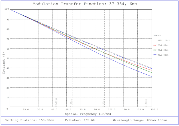
#37-384, 6mm FL f/5.6, Rugged Blue Series M12 Lens, Modulated Transfer Function (MTF) Plot, 150mm Working Distance, f5.6
