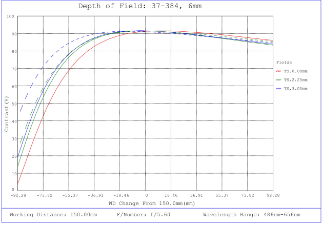
#37-384, 6mm FL f/5.6, Rugged Blue Series M12 Lens, Depth of Field Plot, 150mm Working Distance, f5.6
