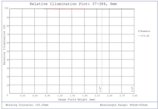
#37-384, 6mm FL f/5.6, Rugged Blue Series M12 Lens, Relative Illumination Plot
