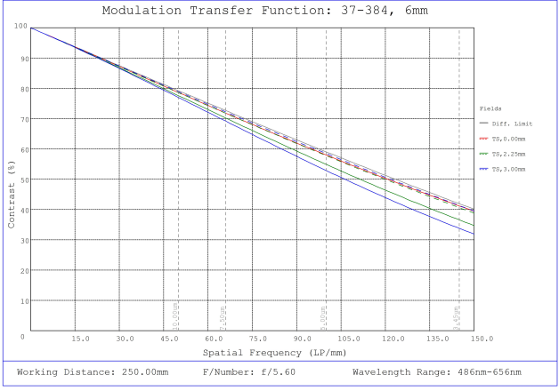
#37-384, 6mm FL f/5.6, Rugged Blue Series M12 Lens, Modulated Transfer Function (MTF) Plot, 250mm Working Distance, f5.6
