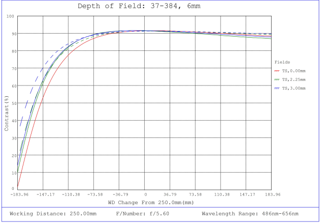
#37-384, 6mm FL f/5.6, Rugged Blue Series M12 Lens, Depth of Field Plot, 250mm Working Distance, f5.6
