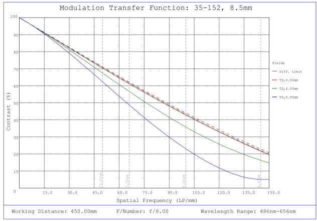
#35-152, 8.5mm, f/8.0, 75mm-∞ Primary WD, HRr Series Fixed Focal Length Lens, Modulated Transfer Function (MTF) Plot, 450mm Working Distance, f8
