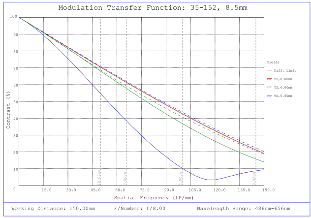
#35-152, 8.5mm, f/8.0, 75mm-∞ Primary WD, HRr Series Fixed Focal Length Lens, Modulated Transfer Function (MTF) Plot, 150mm Working Distance, f8
