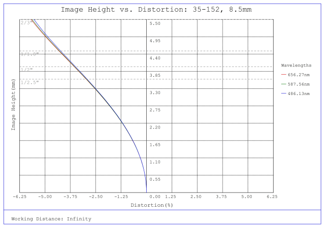
#35-152, 8.5mm, f/8.0, 75mm-∞ Primary WD, HRr Series Fixed Focal Length Lens, Distortion Plot
