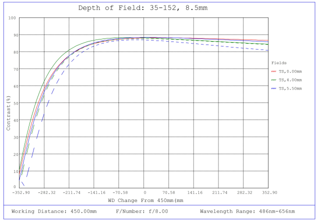
#35-152, 8.5mm, f/8.0, 75mm-∞ Primary WD, HRr Series Fixed Focal Length Lens, Depth of Field Plot, 450mm Working Distance, f8
