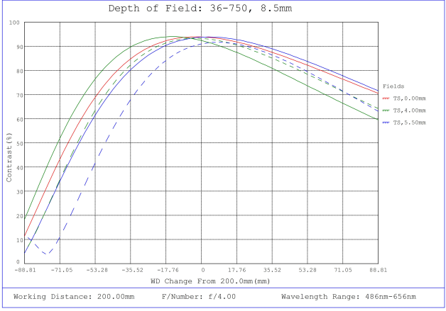
#36-750, 8.5mm f/4, 75mm-∞ Primary WD, HRi Series Fixed Focal Length Lens, Depth of Field Plot, 200mm Working Distance, f4
