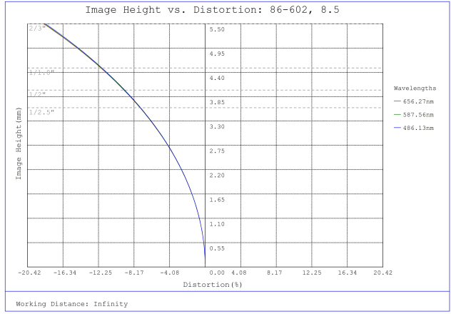
#86-602, 8.5mm, f/4 Ci Series Fixed Focal Length Lens, Distortion Plot
