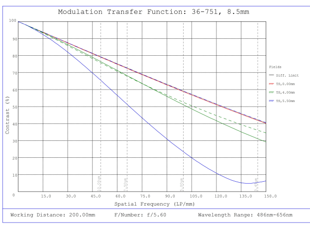
#36-751, 8.5mm f/5.6, 75mm-∞ Primary WD, HRi Series Fixed Focal Length Lens, Modulated Transfer Function (MTF) Plot, 200mm Working Distance, f5.6
