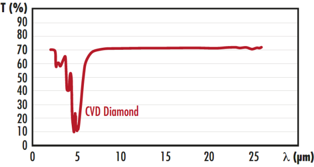
Infrared Windows Transmission
