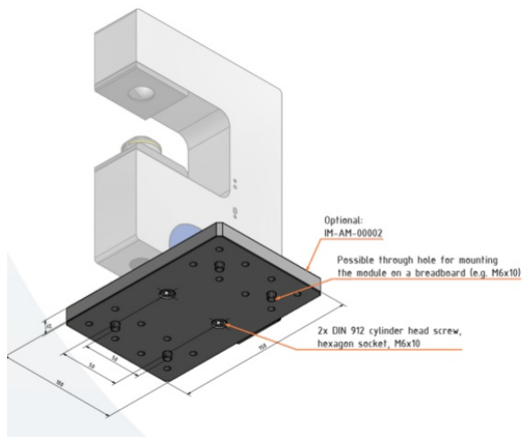
IM-AM-00002 - Adapter plate for mounting on a breadboard
