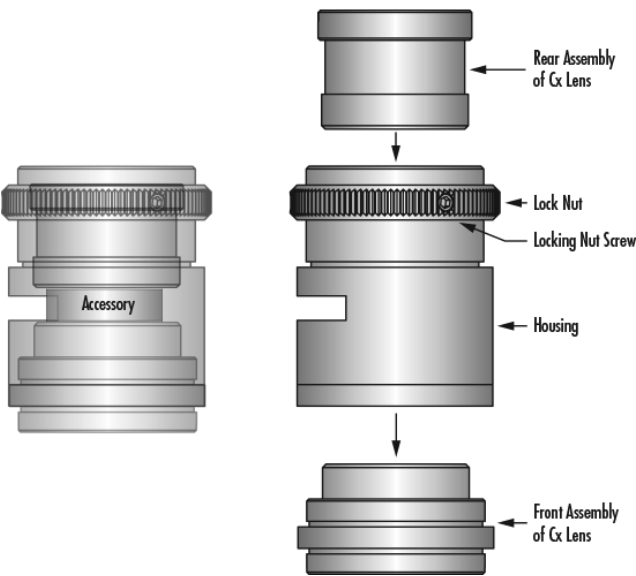
Cx Lens Assembly Diagram
