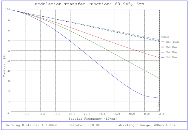
#83-945, f/8, 6mm Focal Length Green Series M12 Lens, Modulated Transfer Function (MTF) Plot, 150mm Working Distance, f8
