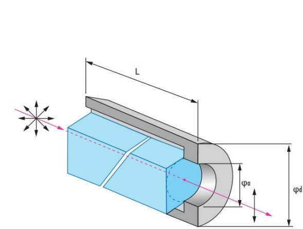
Glan-Taylor Polarizers
