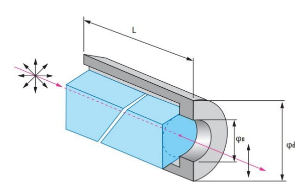
Glan-Taylor Polarizers
