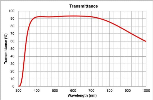
LUCPLFLN20X2 Transmission Graph
