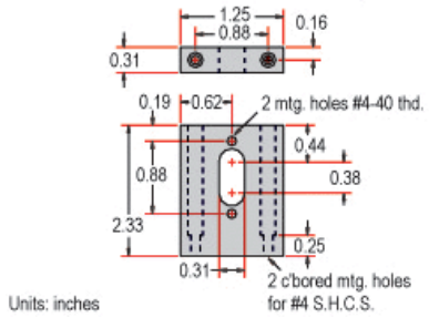
1.25" Z-Axis Adapter Plate (#54-370)
