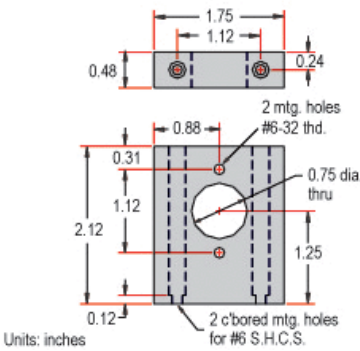
1.75" Z-Axis Adapter Plate (#54-372)
