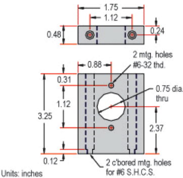
1.75" Z-Axis Adapter Plate (#54-375)
